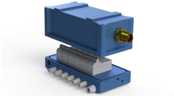
Figure 5 - Pneumatique enclosure
