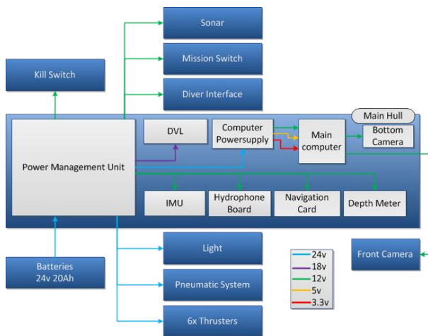
Figure 8 - Power distribution
