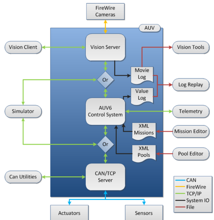
Figure 12 - Software architecture
